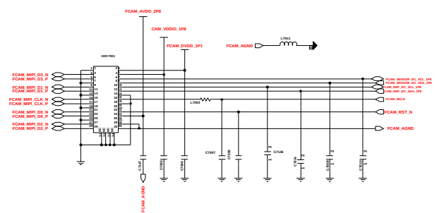
FRONT_16M CAMERA(30PIN)
