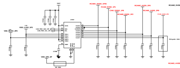
CAM PMIC
