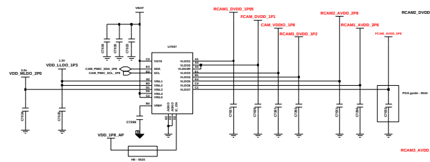
CAM PMIC
